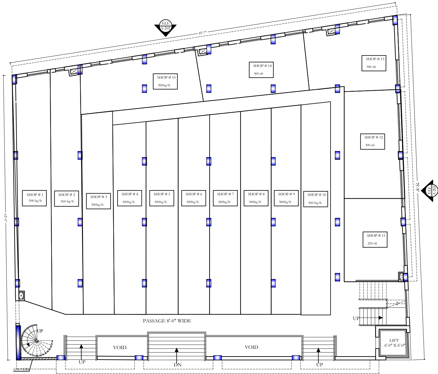
GROUND FLOOR PLAN (Total Area 5698.00 sft.)
